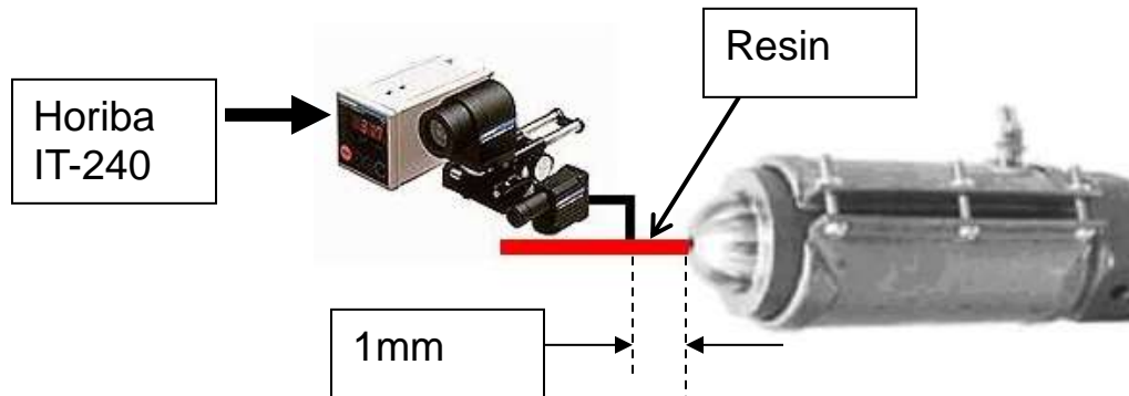
Measurement of Actual Resin Temperature (Material = PBT)
